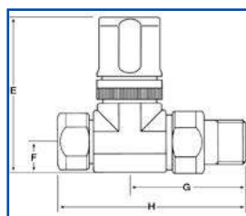
Valvola diritta / Straight valve
